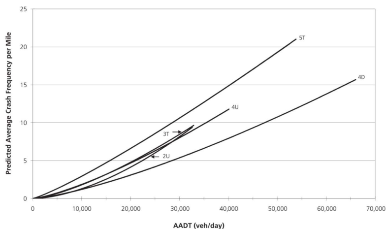
Figure 12-3. Graphical Form of the SPF for Multiple Vehicle Nondriveway collisions (from Equation 12-10 and Table 12-3)
